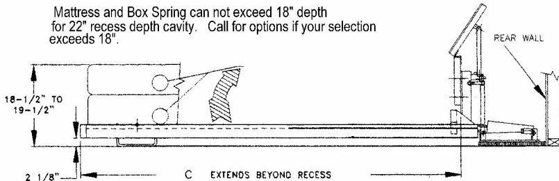
SECTION J-J
